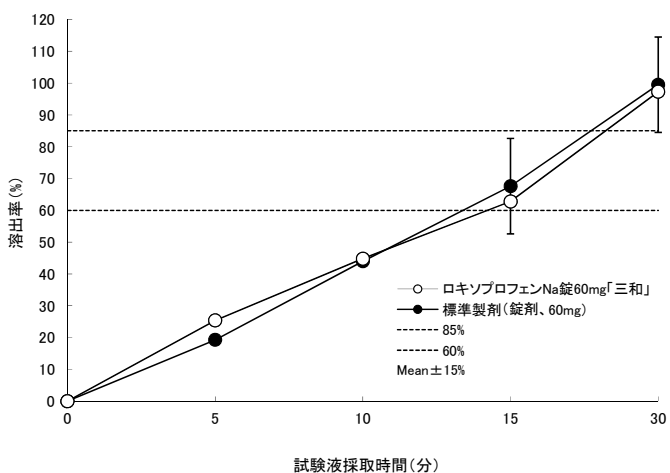
試験液:pH6.8 [判定基準:B]
